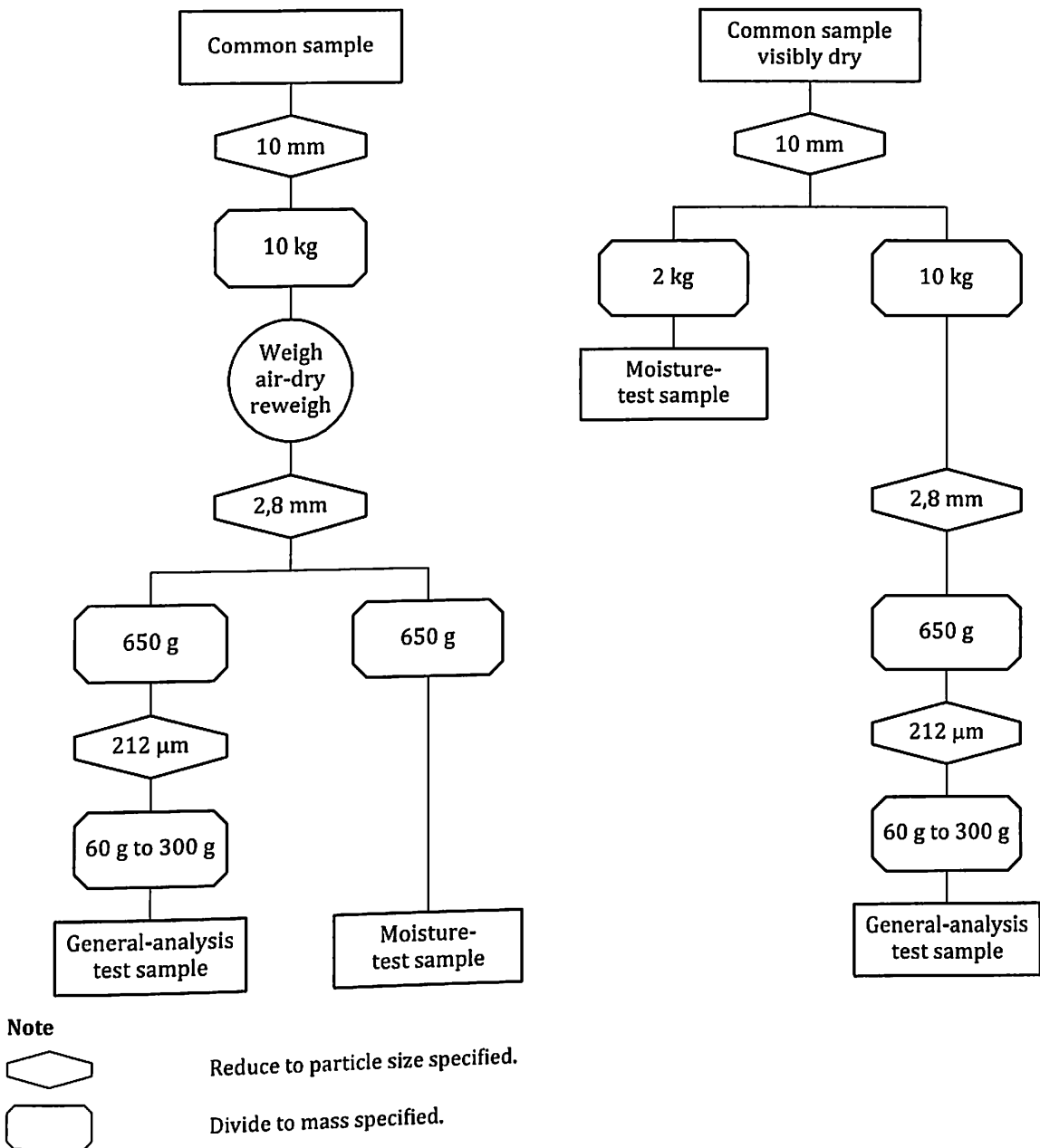
Figure 9 — Examples of preparation of test samples from a common sample for moisture determination and general analysis
