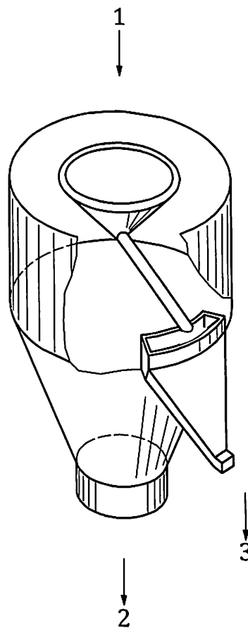
g) Rotating chute type
