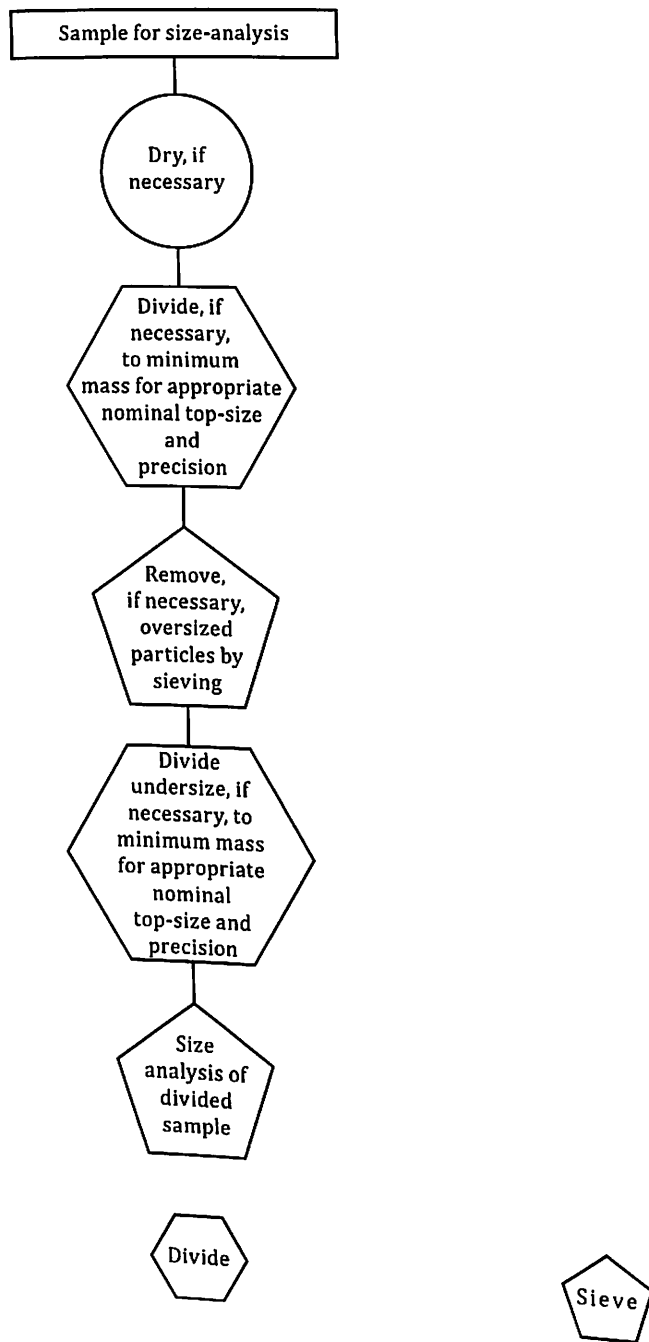
Figure 10 — Example of preparation of samples for size analysis and/or other tests
