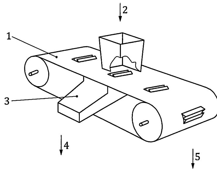
e) Slotted-belt type
