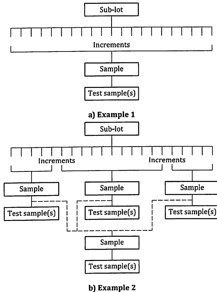
Figure 1 — Examples of the constitution of samples
